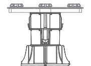
P 9236 + 2x P 9241 + P 9247 min. 145 mm – max. 185 mm
